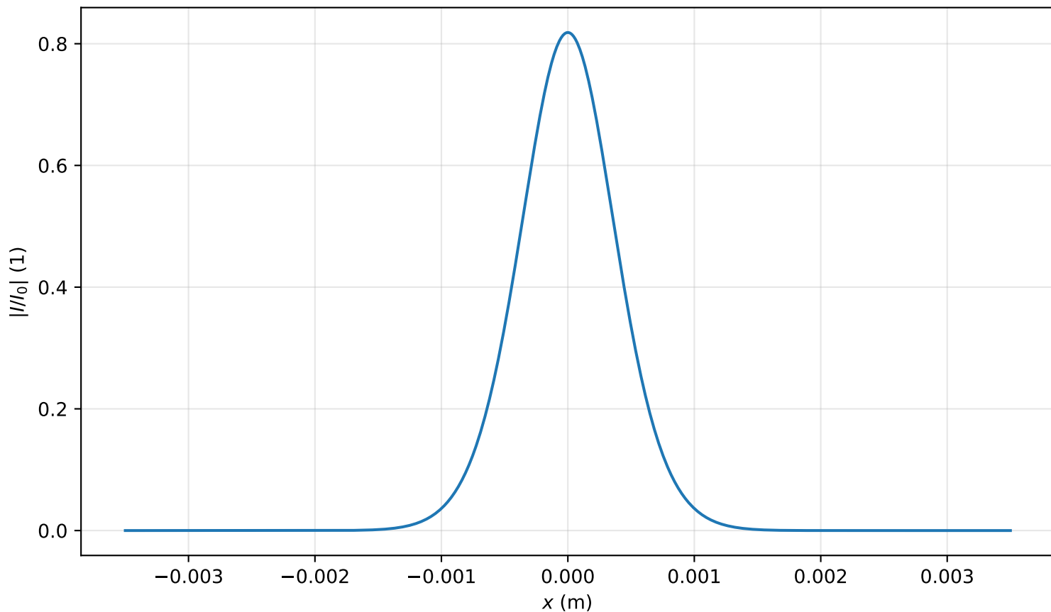
Intensity profile I(x, y = 0, z = 1.433m)/I_0 , P_{in}=0.3P_{cr} , artificial time
